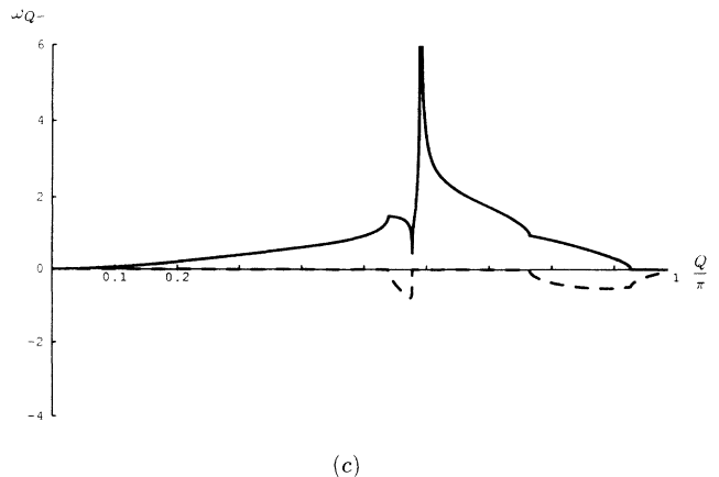
FIG. 2. The nonlinear asymmetric coupler ( \sigma = \infty , \rho = 0 ): (a) \omega_{\Delta Q} vs Q ; (b) \omega_{Q+} vs Q ; (c) \omega_{Q-} vs Q .
